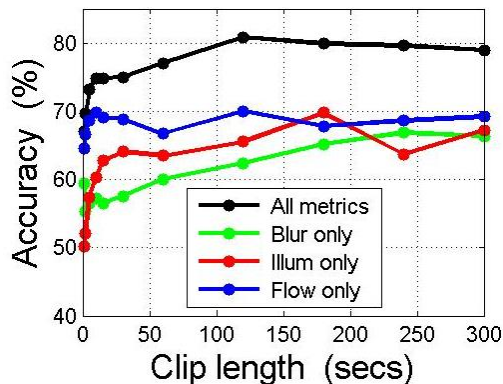
Figure 1. FPV/TPV classifier accuracy as a function of clip length.
